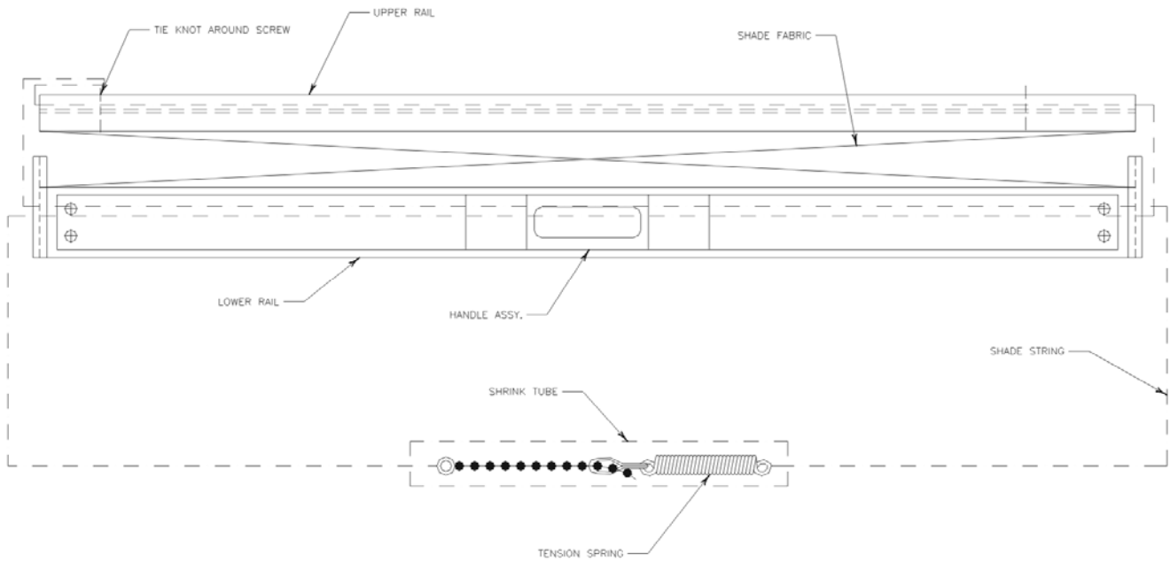
FIGURE 6/ GRAPHIC 25-23-11-991-006
